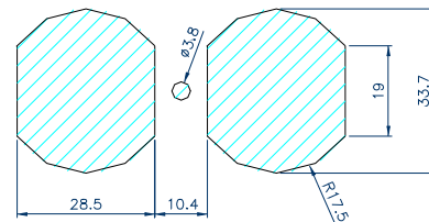
Panel Cutout
