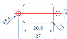
PANEL CUTOUT
