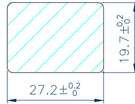
PANEL CUTOUT
