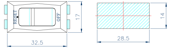
PANEL CUT OUT
