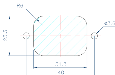
Panel Cut-Out
