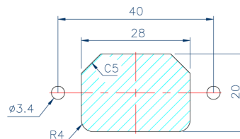
Mounting inlet flange in front of cover.
